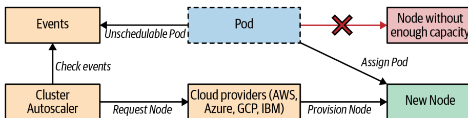
Figure 29-5. Cluster autoscaling mechanism
