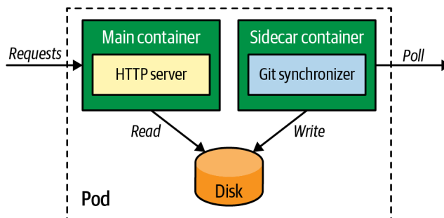
Figure 16-1. Sidecar pattern
